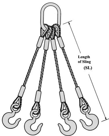
4 Leg Flemish Eye Sling
