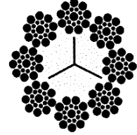
8 x 21 Filler Wire 1/2" diameter and larger
