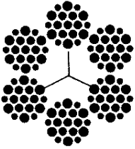
6 x 19 Warrington through 5/16" diameter
