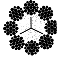
8 x 19 Warrington through 7/16" diameter
