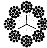
8 x 21 Filler Wire 1/2" diameter and larger
